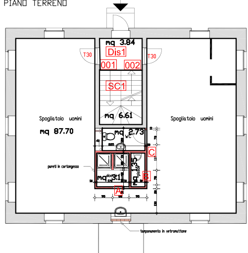
PIANO TERRENO
