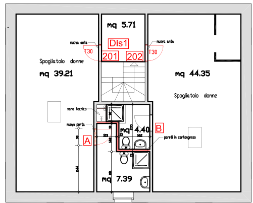
PIANO MANSARDATO
