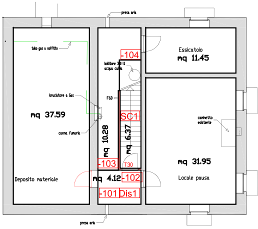
PIANO CANTINATO
