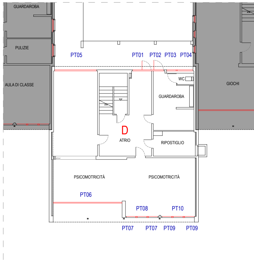
PIANO TERRENO
