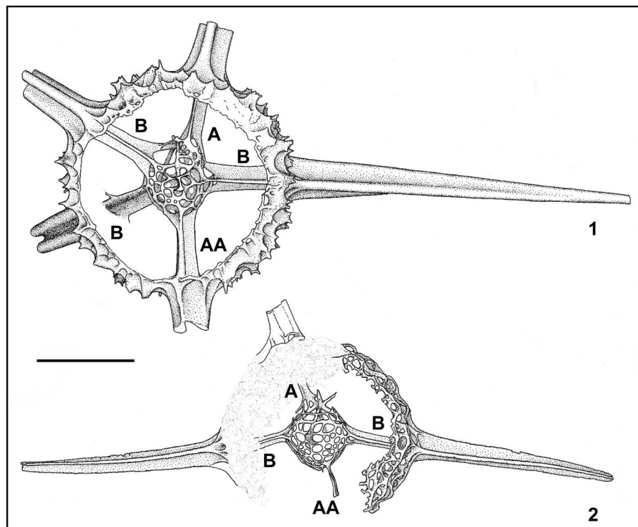
Fig. 10 - Internal structure of Bernoulliella gen. n. 1) Specimen from the S. italicus Radiolarian Zone (late Anisian); sample Rc4, Recoaro, Vicentinian Alps, N Italy, 2) Specimen from the Pelsonian (middle Anisian) of Cristian, Eastern Carpathians, Romania. Cortical shell only partly illustrated. A apical bar, AA antapical bar, B basal bar. Scale bar = 100 \mu m. Drawing by P. Dumitrica.
