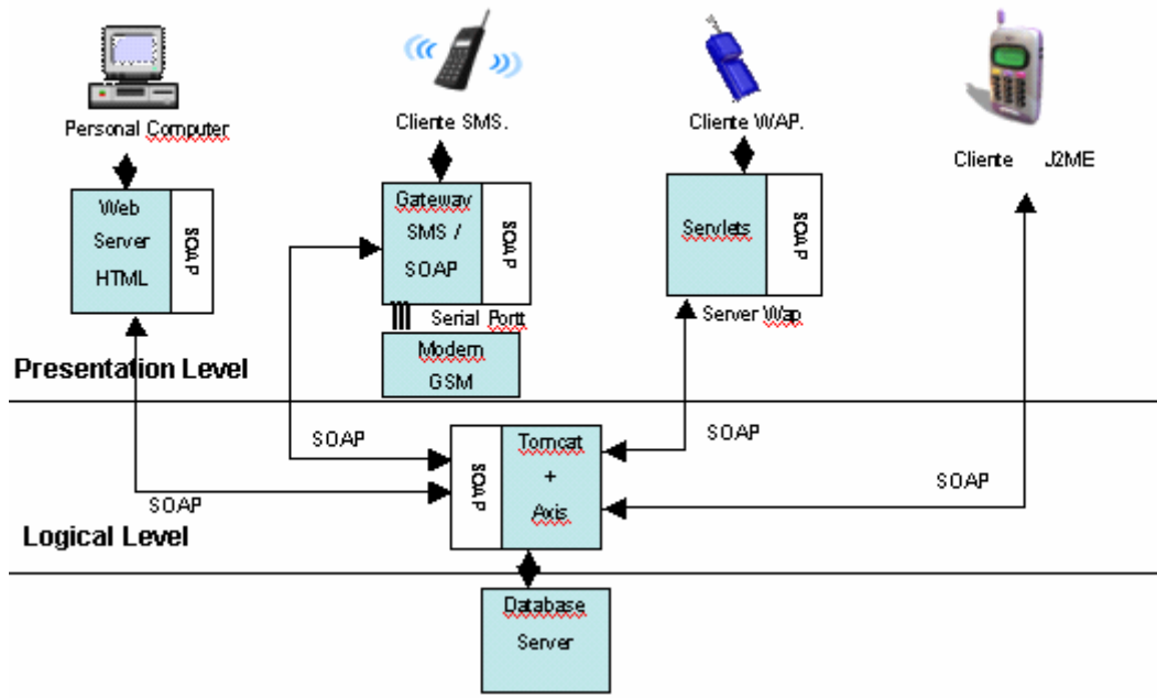
Figure 3. Web services based open architecture.
